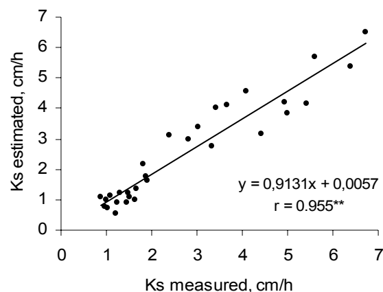
Figure 1. Relationship between measured Ks and Ks values estimated using PTF model 6.
